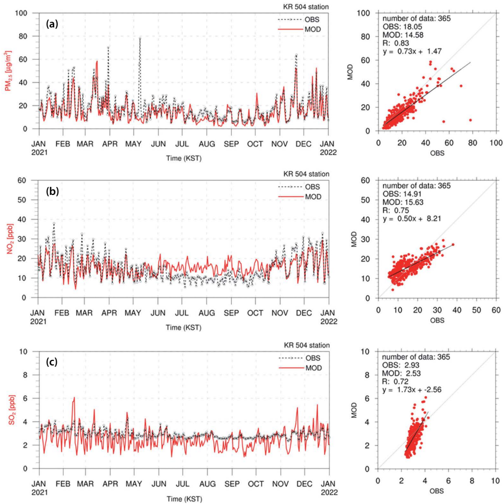
Fig. 3. Daily time series (left) of simulated (red solid line) and observed (black dotted line with circle mark) surface PM_{2.5} concentration (a), NO_2 concentration (b) and SO_2 concentration (c), and scatter plots (right) between observation and simulation in 2021.
