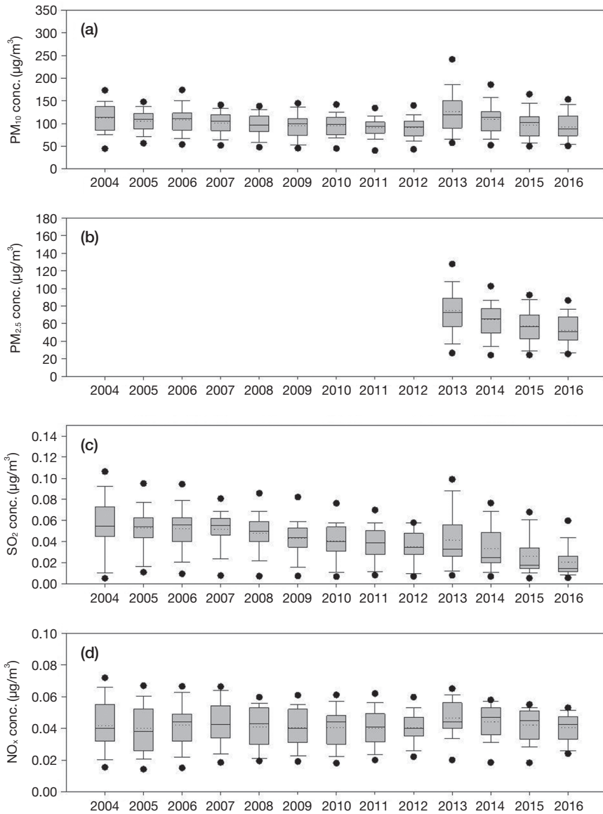
Fig. 6. Annual mean concentration of (a) \text{PM}_{10} , (b) \text{PM}_{2.5} , (c) \text{SO}_2 , (d) \text{NO}_x from 2004 to 2016 (NBS, 2004c-2017c).
