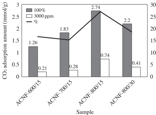
Fig. 9. Comparison of CO 2 adsorption amount 100% with 3000 ppm.
