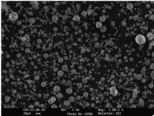
Fig. 4. SEM image of test ash dust : without magnet (× 1000).
