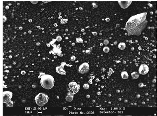
Fig. 2. SEM image of raw ash particles (× 1000).
