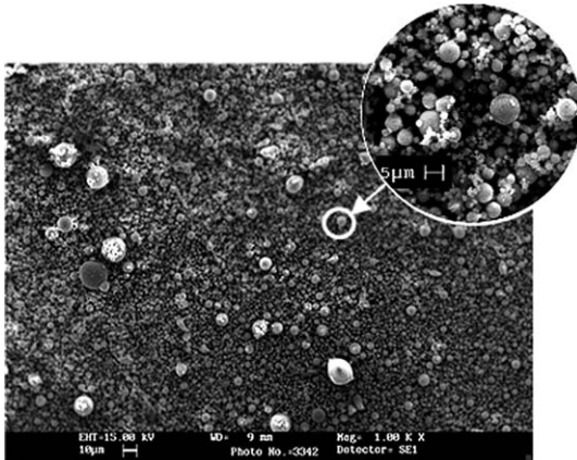
Fig. 5. SEM image of test captured ash dust (× 1000).
