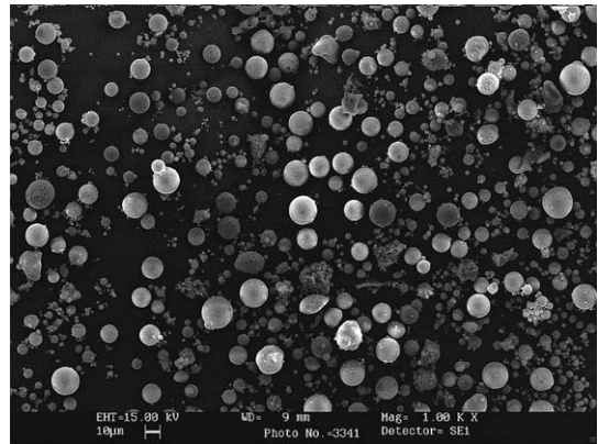
Fig. 3. SEM image of test ash dust (× 1000).
