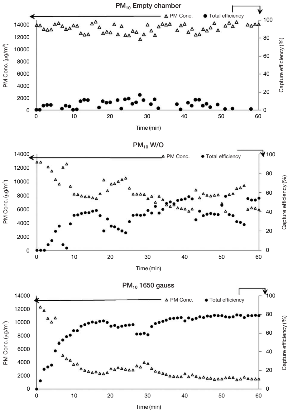
Fig. 10. Magnetic capture of test dust; PM 10 and PM 2.5 in terms of magnetic intensity.
