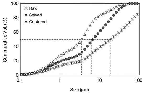
Fig. 6. Cummulative size distribution of raw, seived and captured ash dust.
