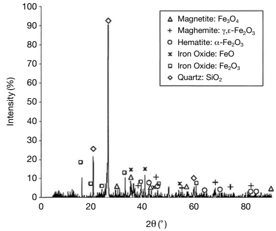
Fig. 7. XRD pattern of test fly ash dust.
